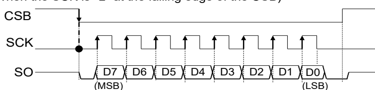
Command data output timing: SCK rising edge operation (When the SCK is "L" at the falling edge of the CSB)
